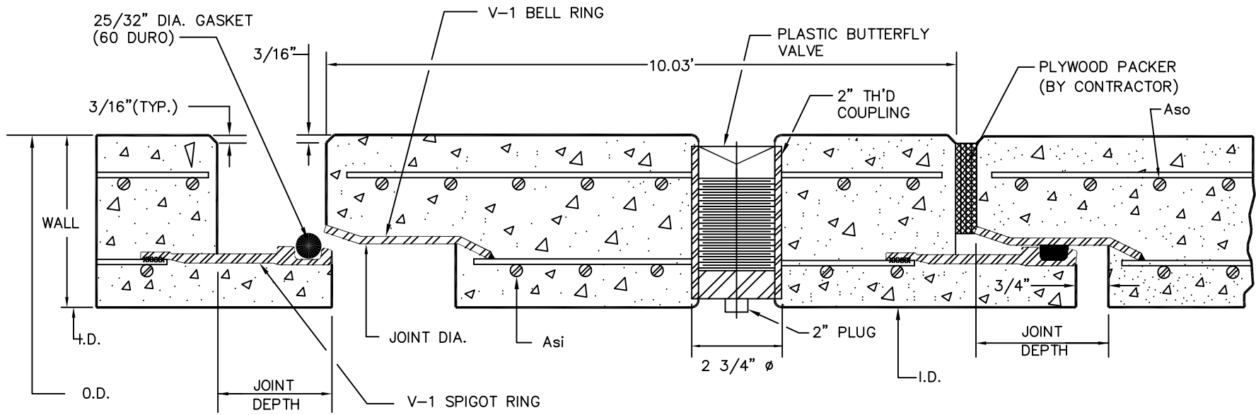
2" GROUT HOLE DETAIL (WITH PLUG)
