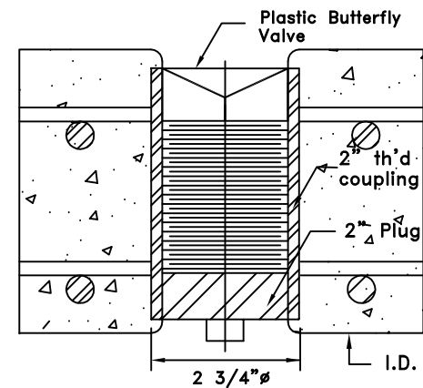
2" GROUT HOLE DETAIL
